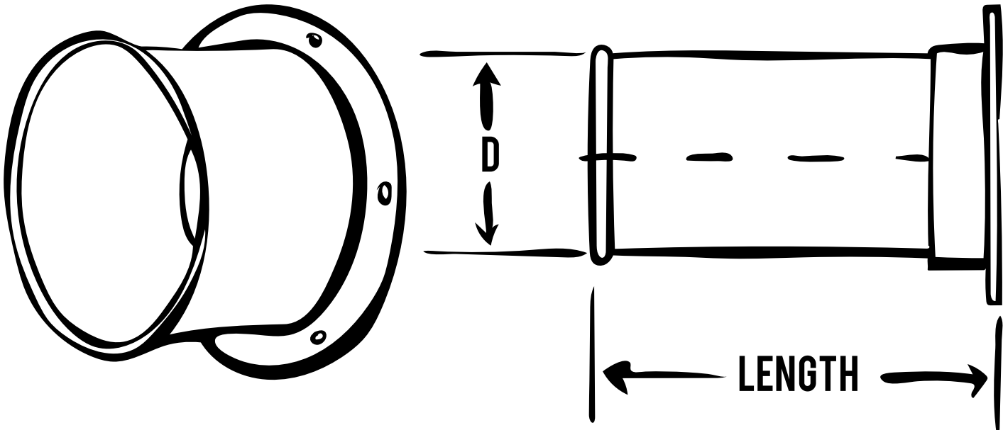
QUICK-FIT ANGLE FLANGE ADAPTER
