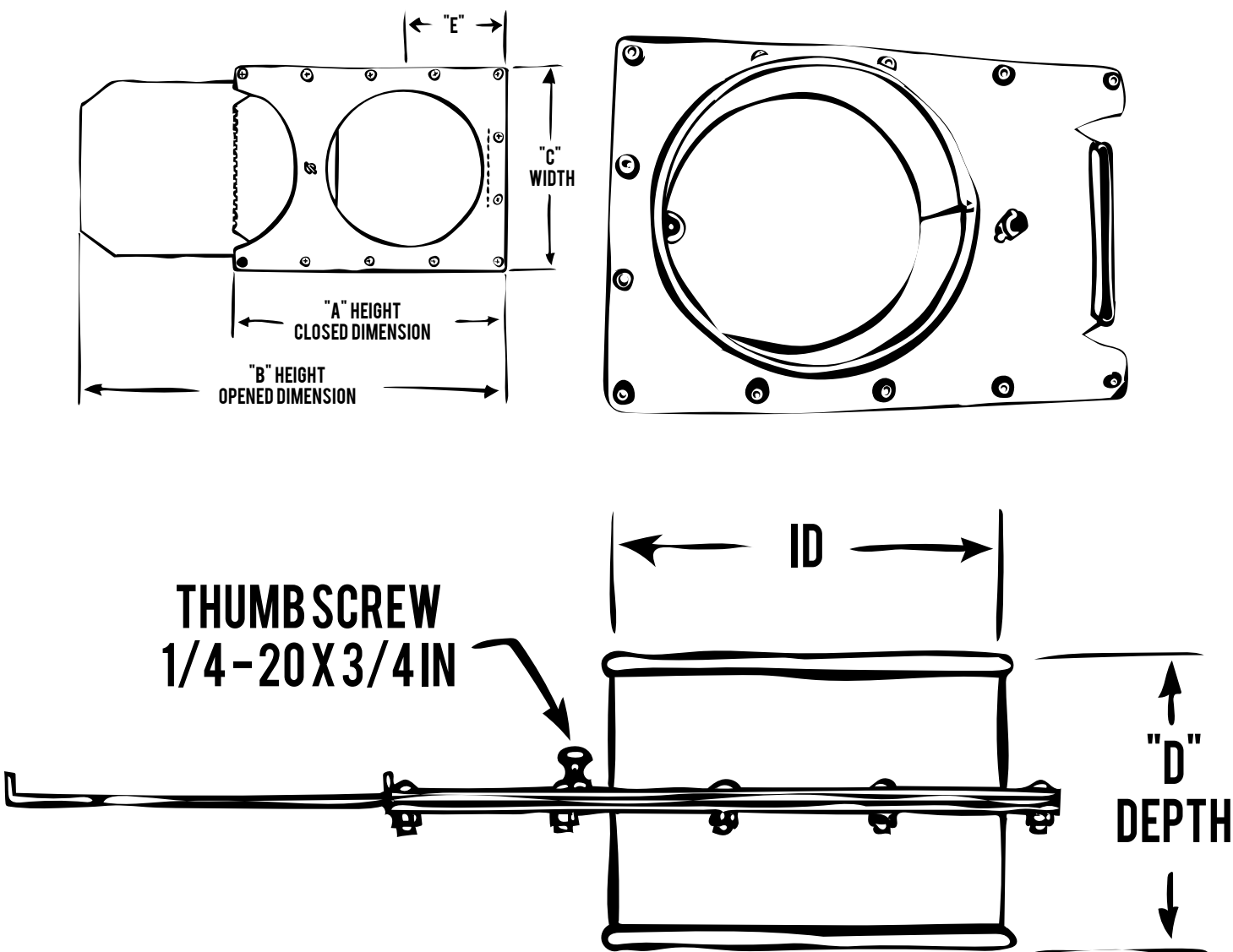
QUICK-FIT MANUAL BLASTGATE
