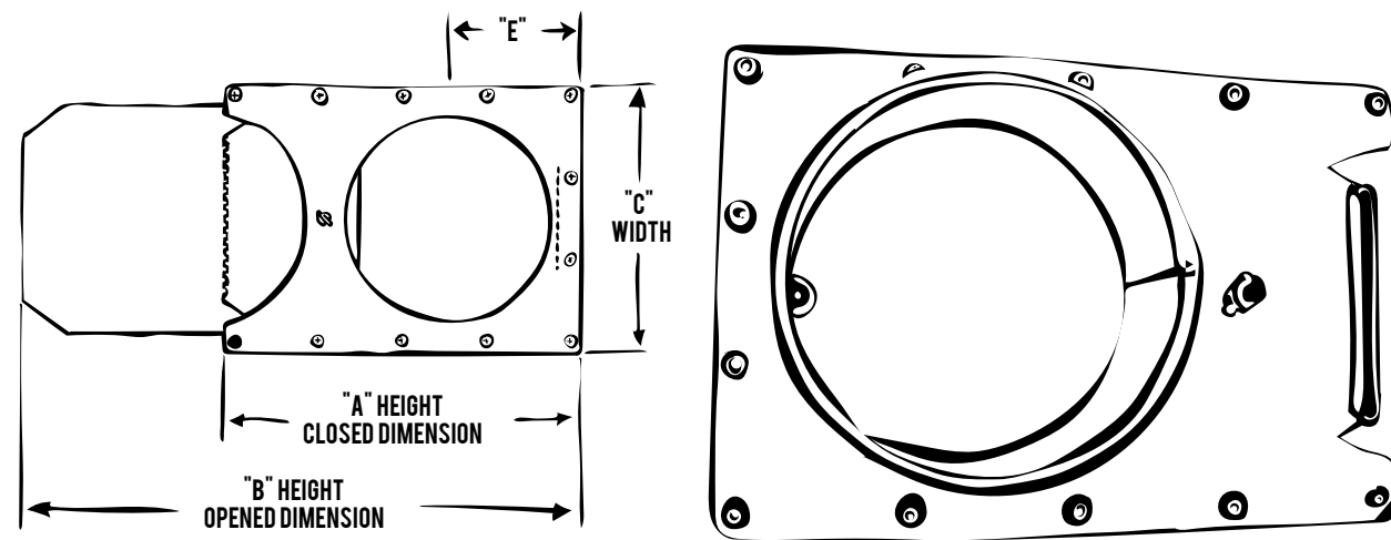
QUICK-FIT MANUAL BLASTGATE
