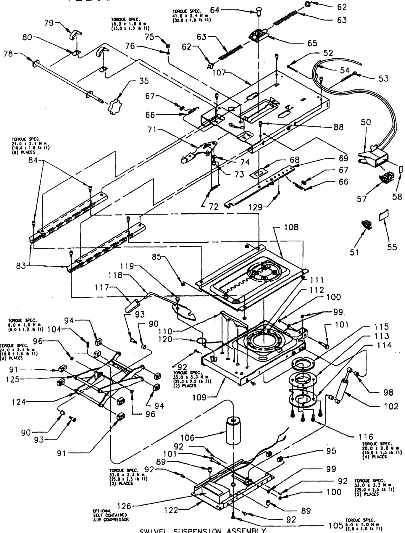
SWIVEL SUSPENSION ASSEMBLY
